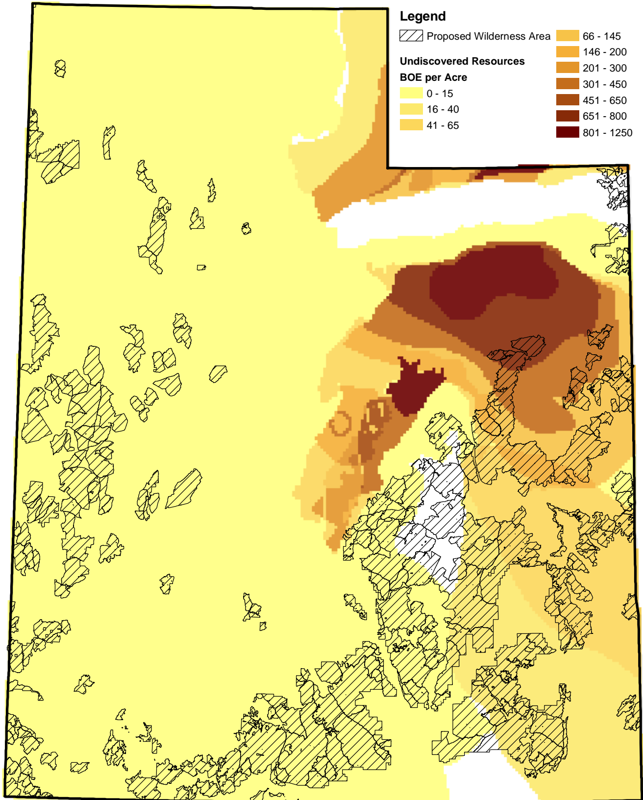
Figure 8: Undiscovered Oil and Gas Resources in Utah
